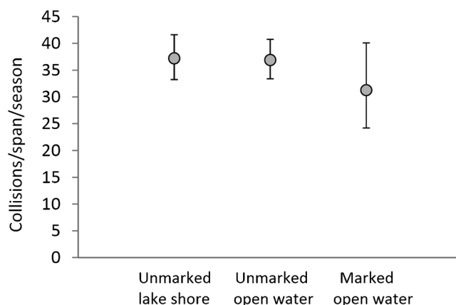
Figure 4. Model-averaged predicted carcasses per span per season (mean and 95% CI) based on avian carcasses that were attributed to power-line collision, vehicle collision, and unidentified cause of death during study of avian collision with power lines conducted from 2006 to 2008 in central North Dakota, USA.
